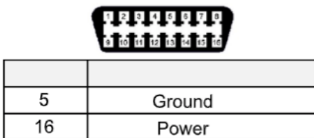
Figure 1 - Vehicle OBDII Connector
